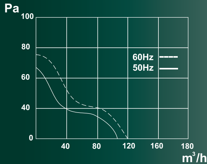
Performance curves
